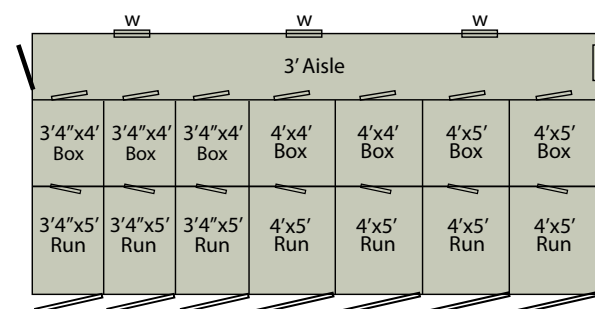
12' x 26' 7-Run Layout
